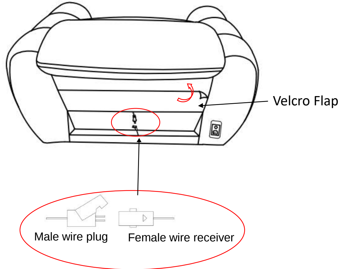
Power headrest Connection
