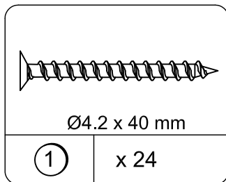
SCREW TCS1012
