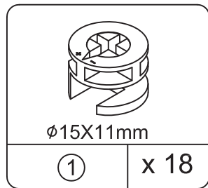
① x 18 CAM LOCK Tornillo De Cerradura SERRURE DE CAME TEL5001
