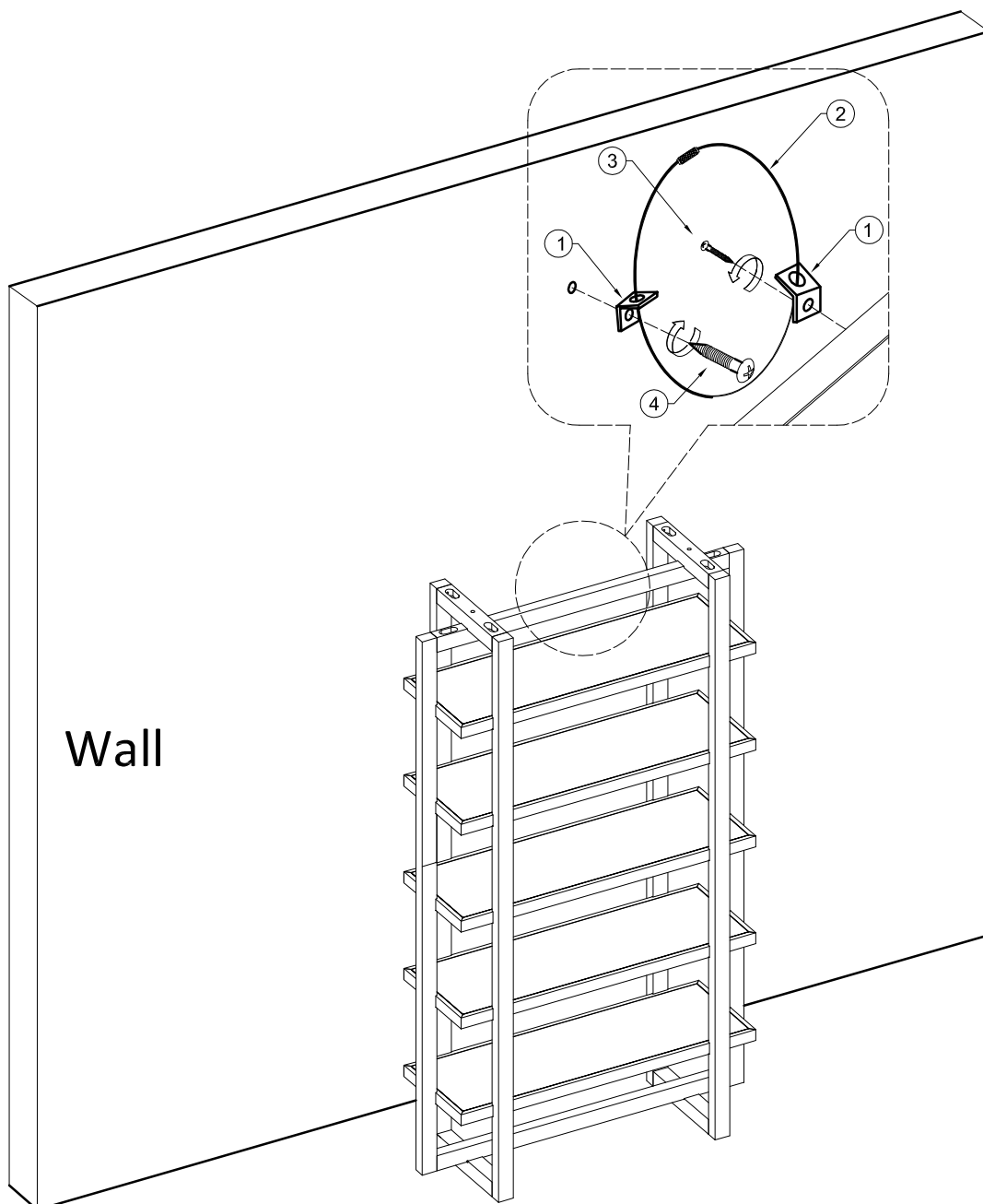
Long Screw 1X
