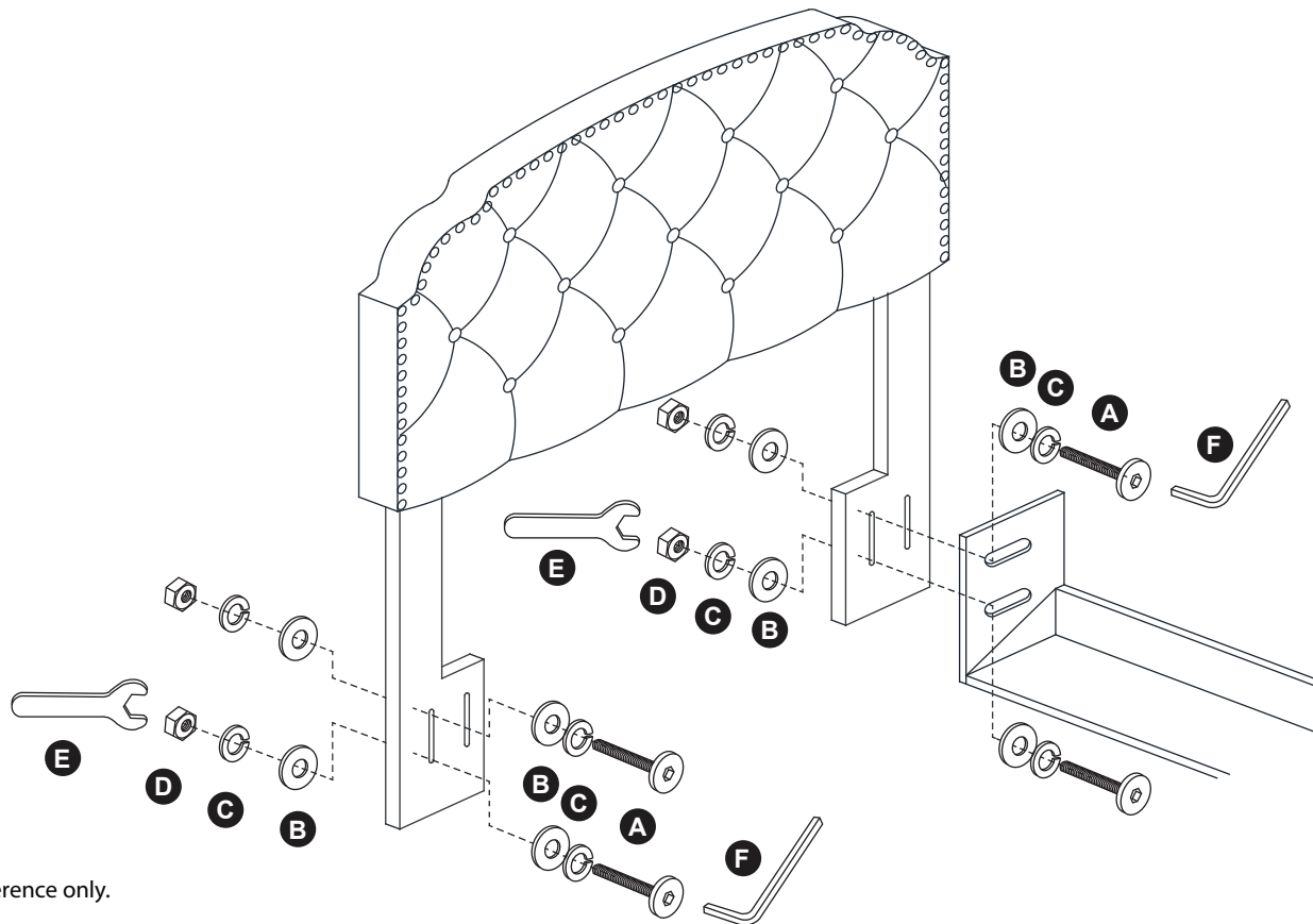
C x8 Spring Washer
