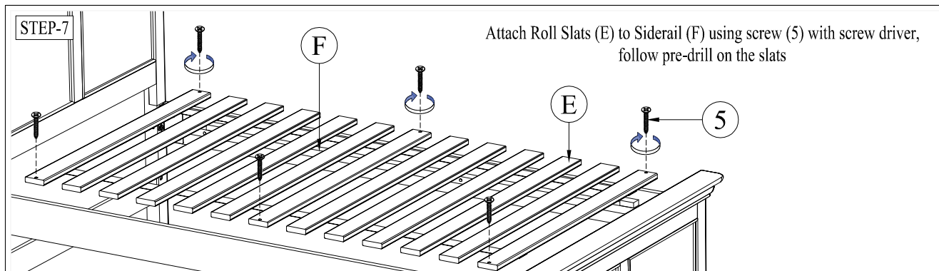
TWIN PANEL BED ASSEMBLY COMPLETE OPTION 1
