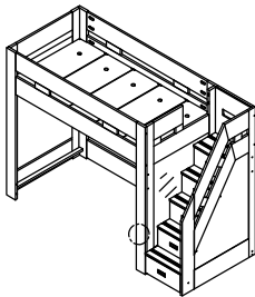
TWIN - FULL LOFT BED W/STAIRCASE (1 OPEN, 1 CLOSED END)
