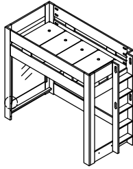
TWIN - FULL LOFT BED W/LADDER (1 OPEN, 1 CLOSED END)
