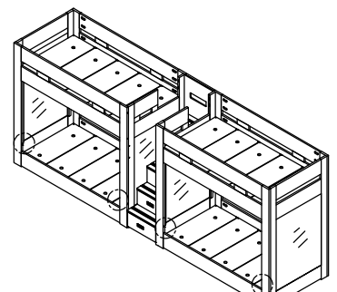
TWIN/TWIN - FULL/FULL DOUBLE BUNK W/STAIRCASE (ALL CLOSED ENDS)
