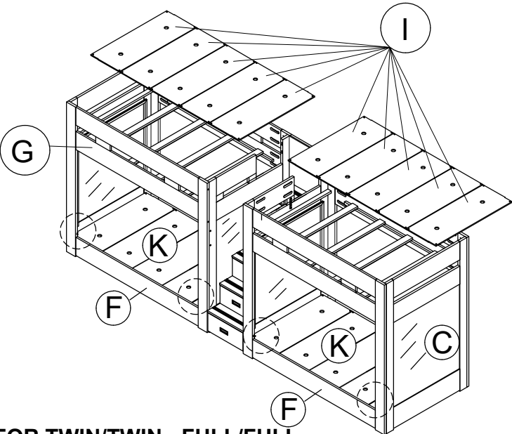
FOR TWIN/TWIN - FULL/FULL DOUBLE BUNK W/STAIRCASE (ALL CLOSED ENDS)
