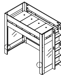
TWIN - FULL LOFT BED W/LADDER (2 CLOSED ENDS)
