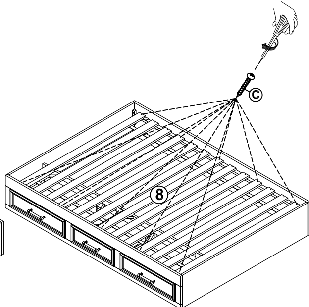
FULL PLATFORM BED
