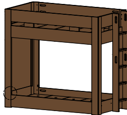
H TWIN/TWIN - FULL/FULL BUNK BED W/LADDER (1 OPEN, 1 CLOSED END)
