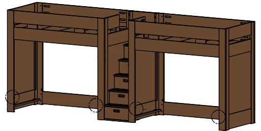
F TWIN / FULL DOUBLE LOFT W/STAIRCASE (ALL CLOSED ENDS)
