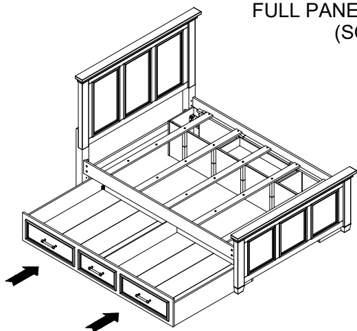
OPTION 1: The trundle in left position
