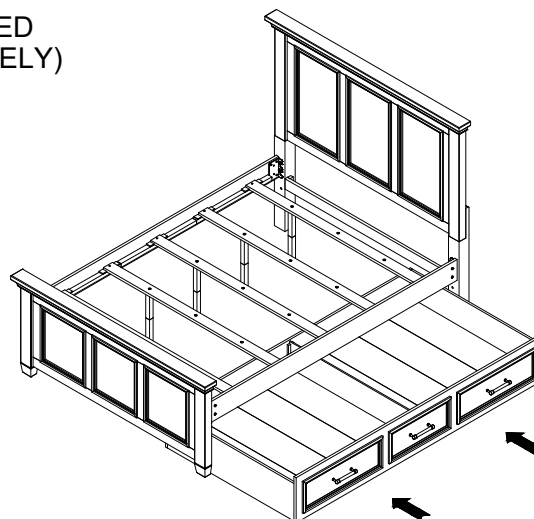
OPTION 2: The trundle in right position
