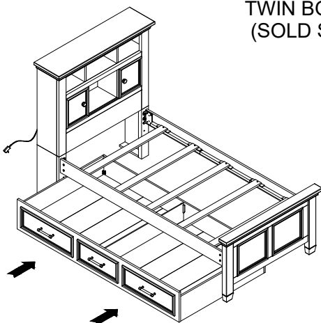
OPTION 1: The trundle in left position
