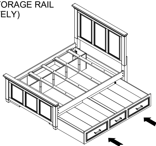
OPTION 2: The trundle in right position
