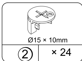
CAM LOCK TLW2019
