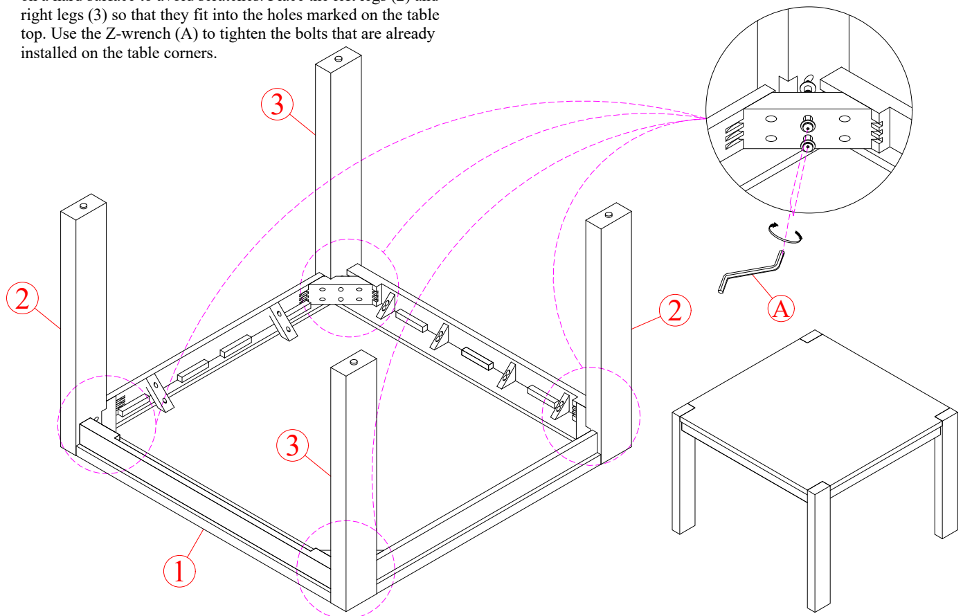
COMPLETE ASSEMBLY
