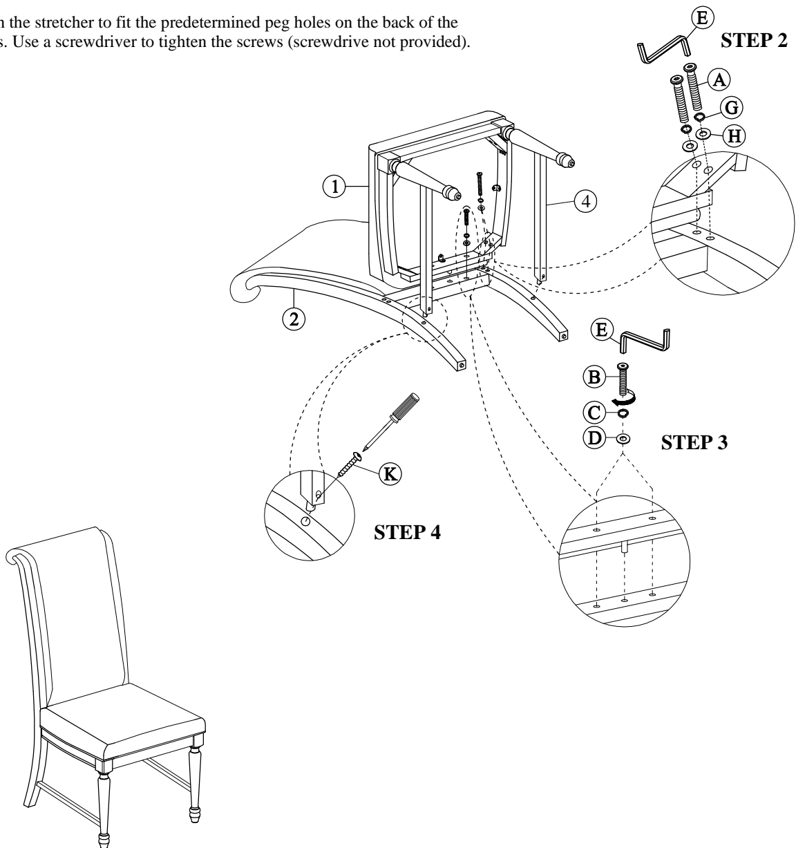
COMPLETE ASSEMBLY
